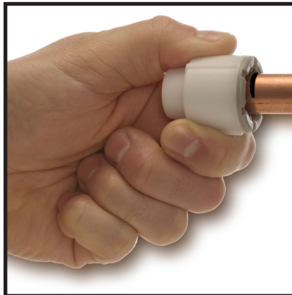
Just mark the pipe 1 1/4", PUSHON, test, twist off and re-use!
